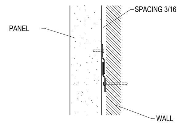
WALL ANCHORING DETAIL
