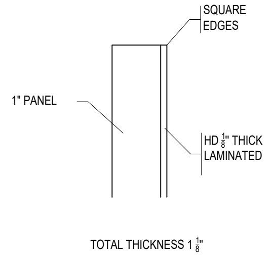
SIDE PANEL DETAIL NO FABRIC
