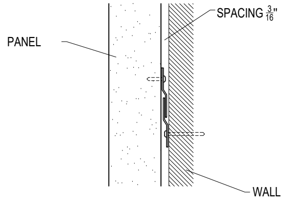
WALL ANCHORING DETAIL SCALE: 3" = 1'-0"
