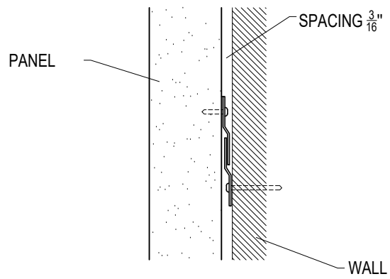
WALL ANCHORING DETAIL
